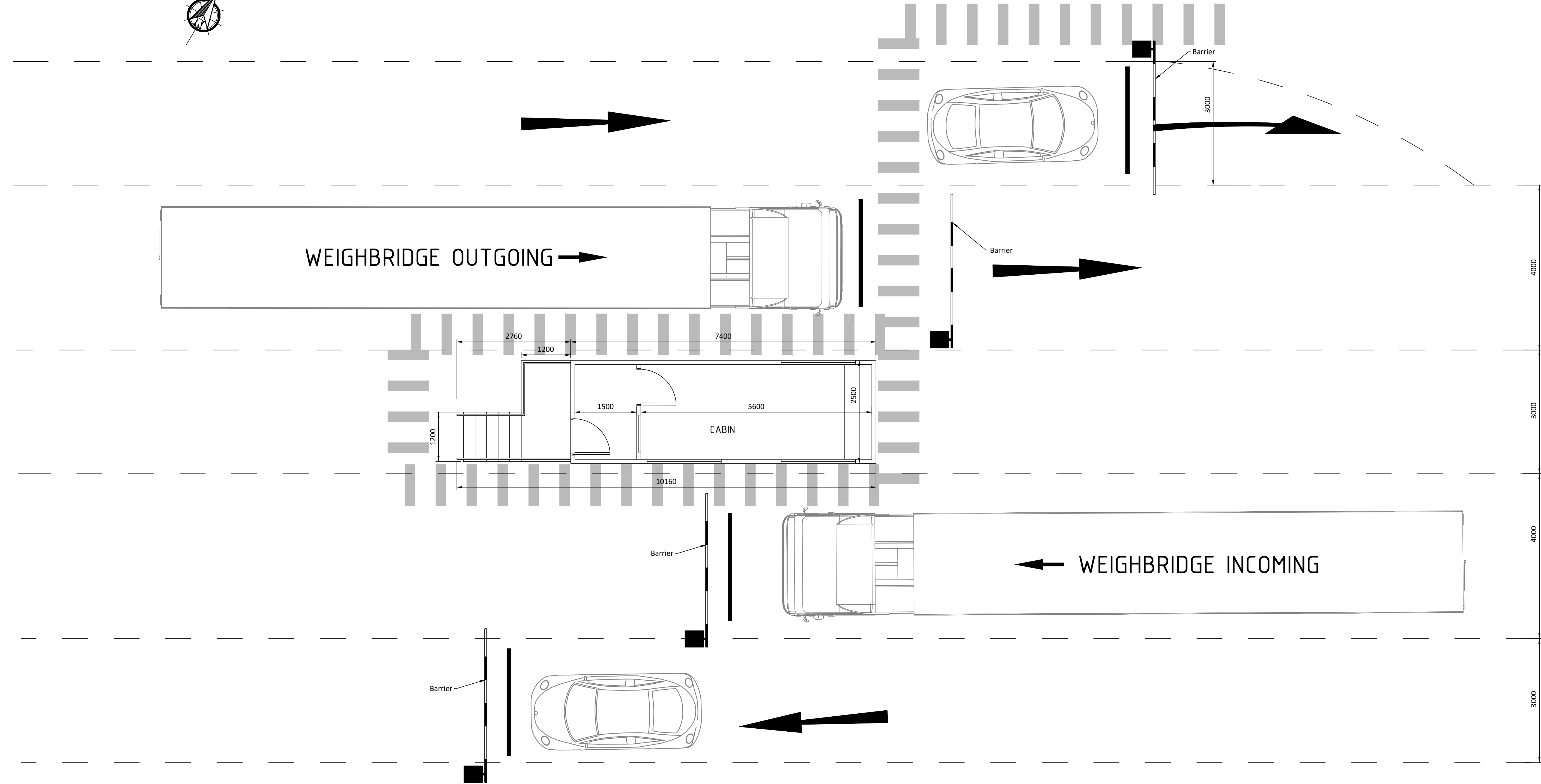
WEIGHBRIDGE PLAN Scale 1:50
